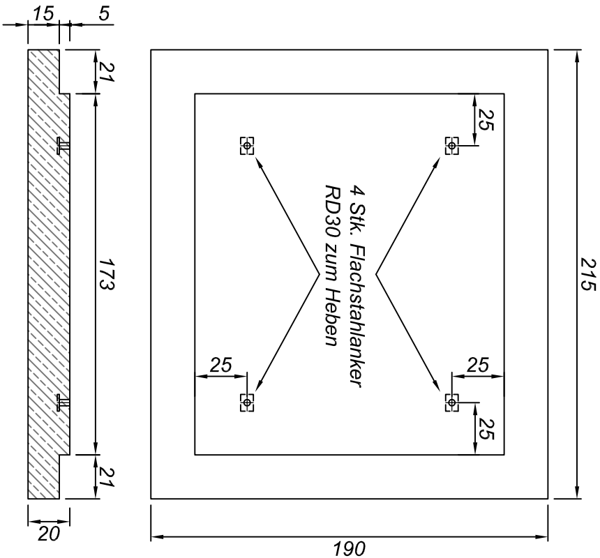
④ Bodenplatte 1Stk.
